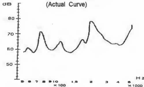
BRT1207P-01-SEHC (Actual Curve)
