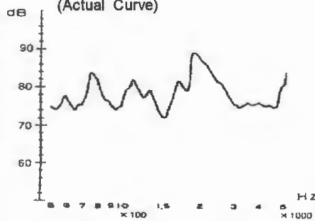
FREQUENCY RESPONSE BRT1207P-01-SEHA (Actual Curve)
