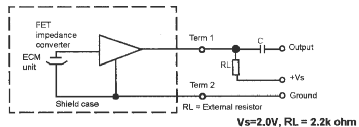
Schematic Diagram:
