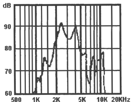
TYPICAL SPL VS. FREQUENCY: BST1310SM-05
