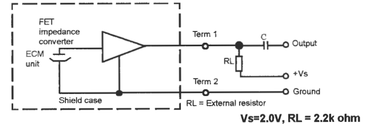
Schematic Diagram:
