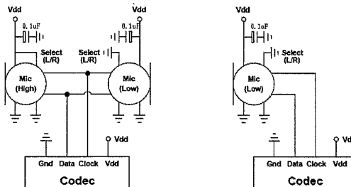
Double MIC
