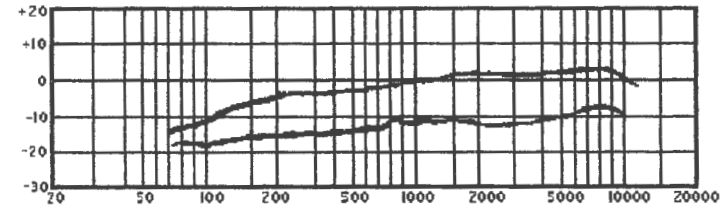
Typical Frequency Response Curve:
