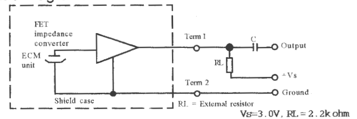
Schematic Diagram:
